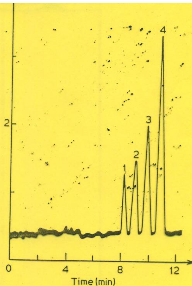
Fig. 16.4 Separation of aflatoxin standards. Column packing, \mu Porasil ( 10\ \mu\text{m} ); column dimensions, 300 \times 4\ \text{mm i.d.} ; eluent, water-saturated dichloromethane/methanol (99.4:0.6); flow rate, 1.05\ \text{ml min}^{-1} ; column temperature, 20^\circ\ \text{C} ; detection system, fluorimeter with cell filled with purified silica ( 100\text{--}200\ \mu\text{m} ). Solutes: 1, aflatoxin \text{B}_1 ; 2, aflatoxin \text{G}_1 ; 3, aflatoxin \text{B}_2 ; 4, aflatoxin \text{G}_2 ( 2.4\ \text{ng} of each). Reproduced with permission from reference 679.
